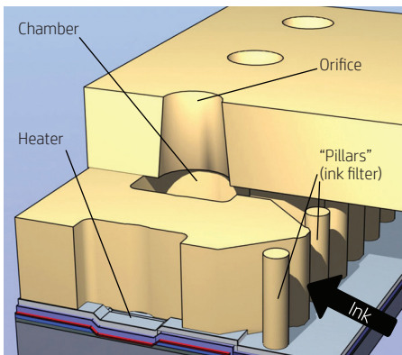
Figure 1 Cutaway view of an HP Thermal Inkjet drop generator
