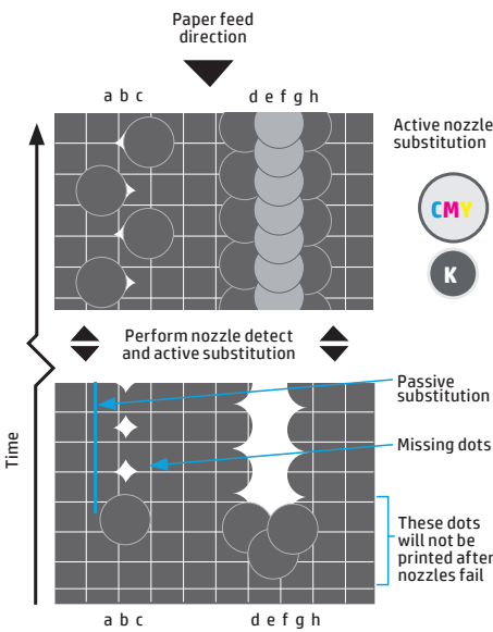
Figure 7 Schematic: nozzle substitution
