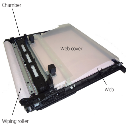
Figure 8: Printhead service station cassette
