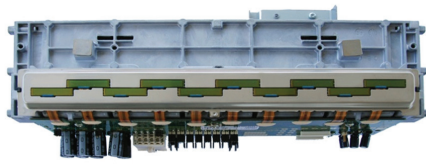
Figure 4 Pagewidth writing engine assembly, bottom view
