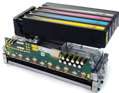
Figure 3 Pagewide writing engine assembly
