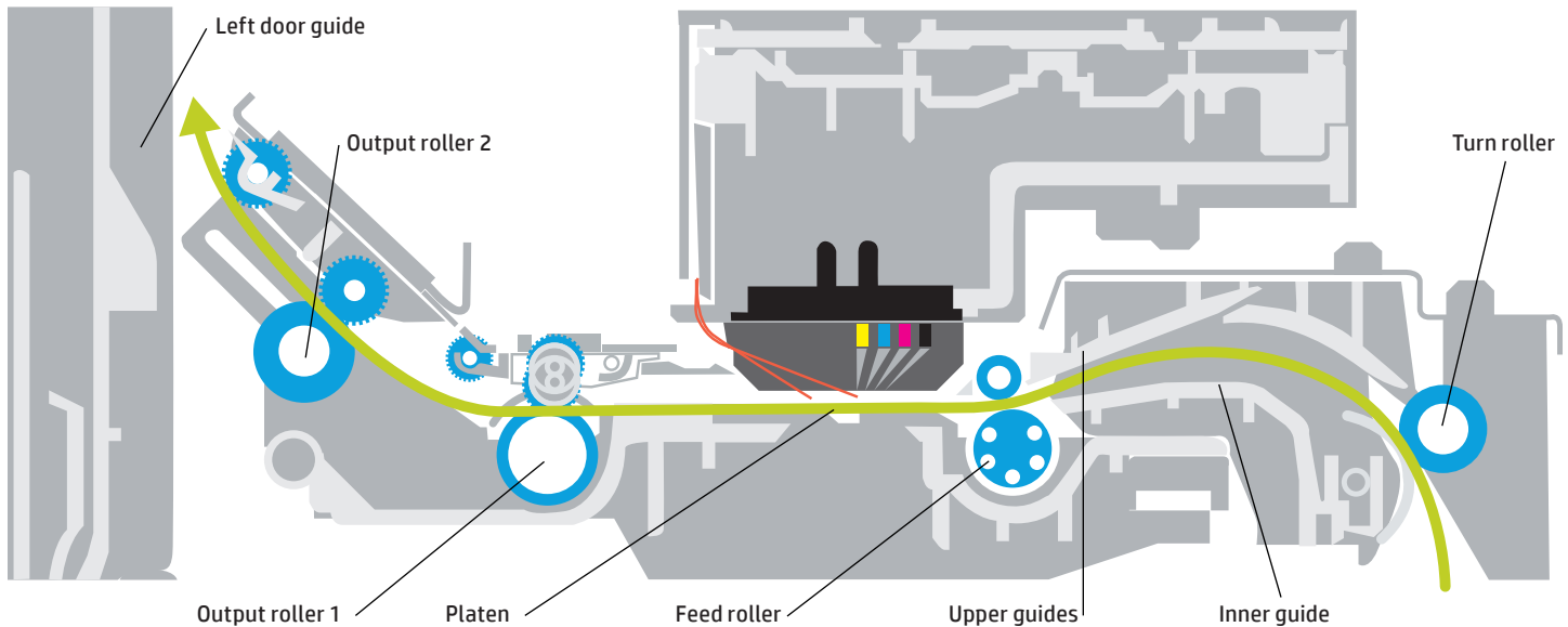
Figure 9: Cross-section of the paper transport
